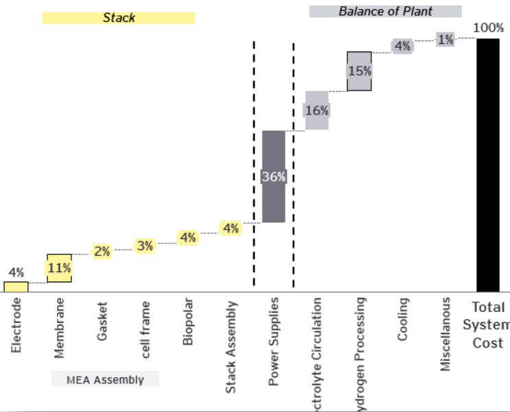
Alkaline Electrolyzer componentwise cost break up -$/kW 1MW @ 10 units/yr production rate
