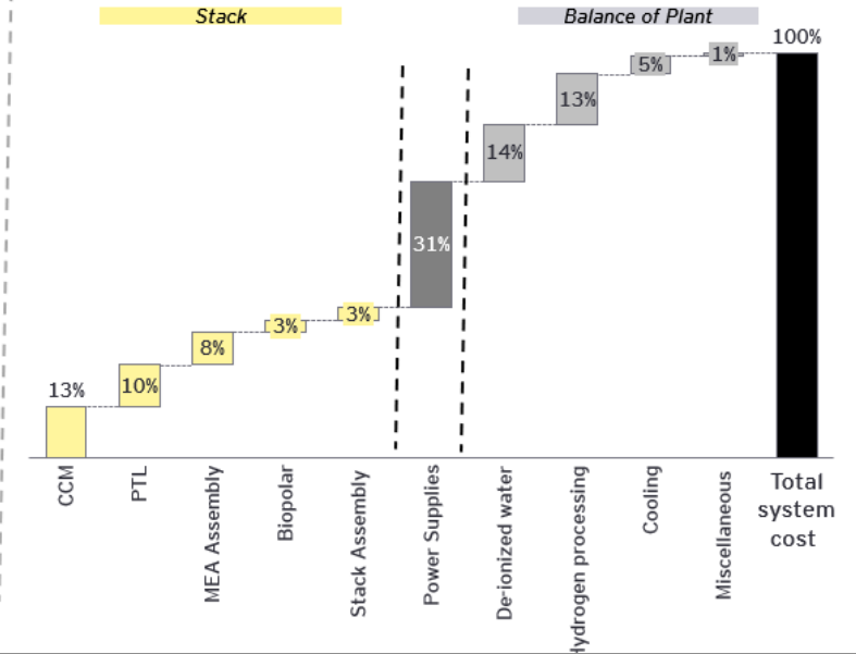
PEM Electrolyzer component wise cost break up (1MW) -$/kW 1MW @ 10 units/yr production rate
